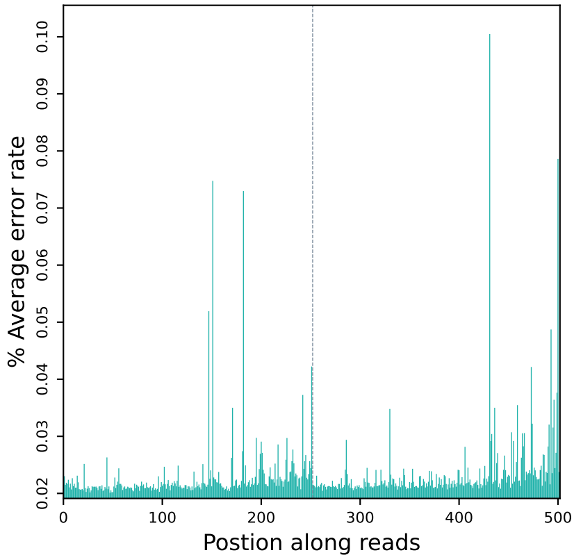
Error rate distribution along reads (R10323)
